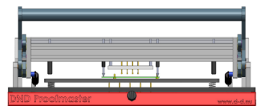
Probes contacting both top and bottom of PCB.
